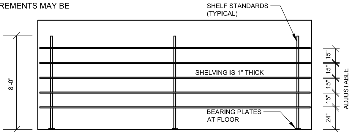
SHELF ELEVATION VIEW
