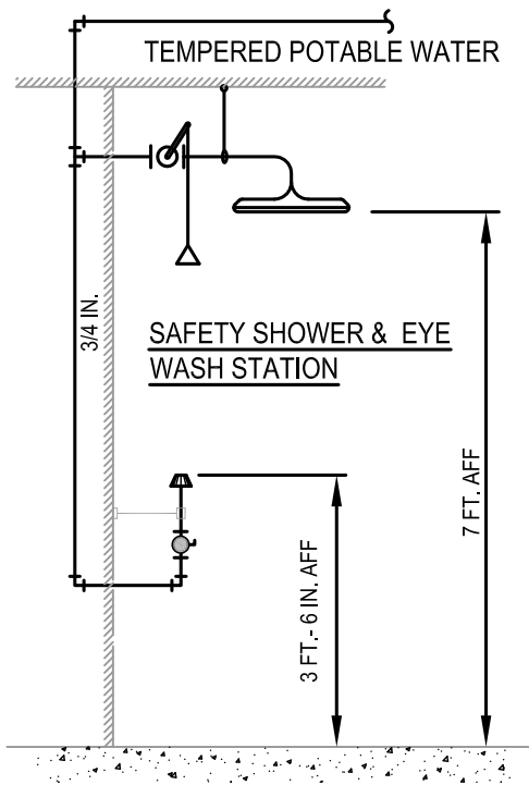
SIDE VIEW SCHEMATIC
