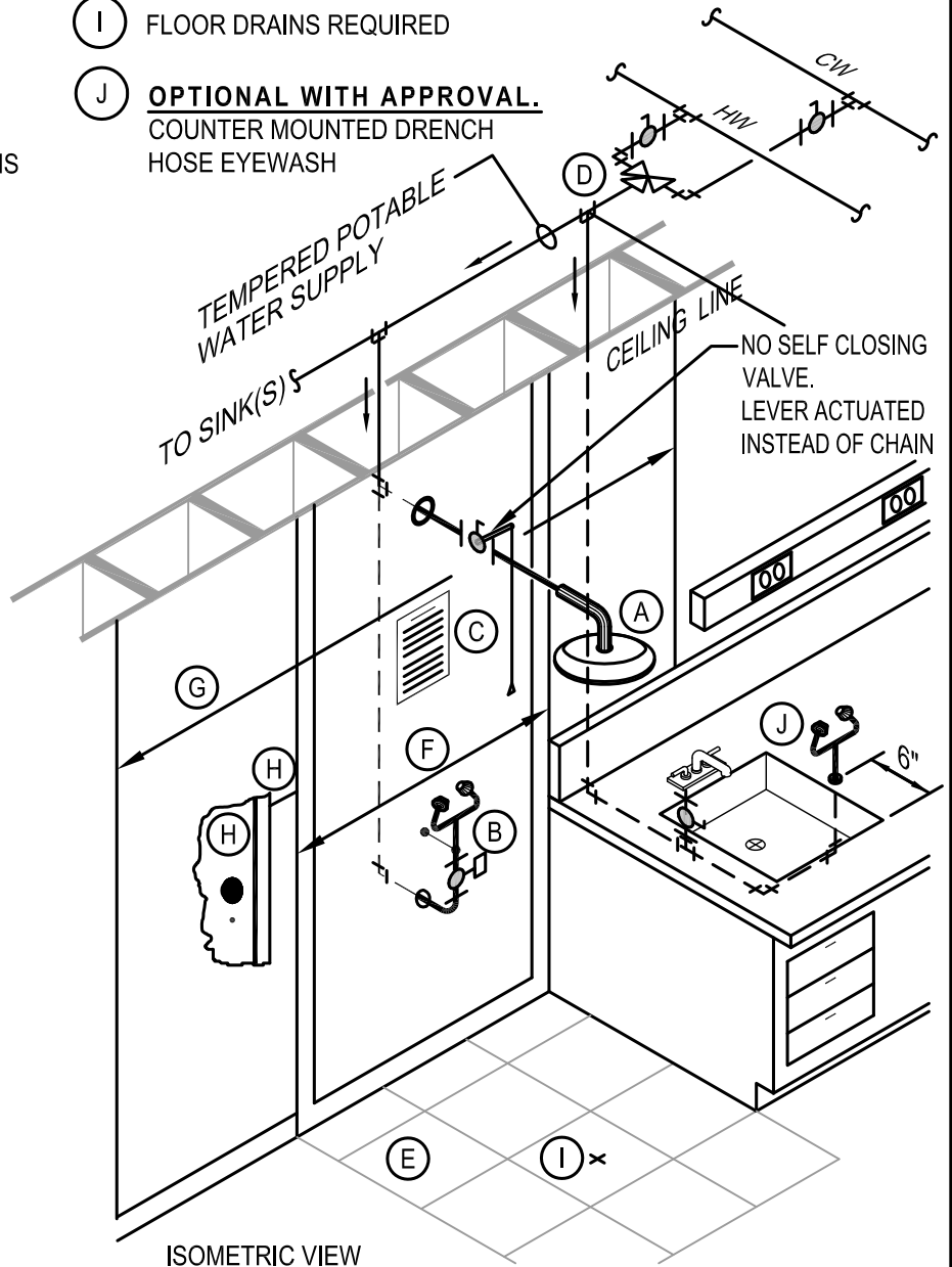
ISOMETRIC VIEW
