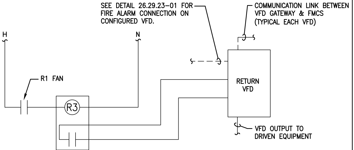
RETURN/ EXHAUST FAN VFD TEMPERATURE CONTROL DIAGRAM
