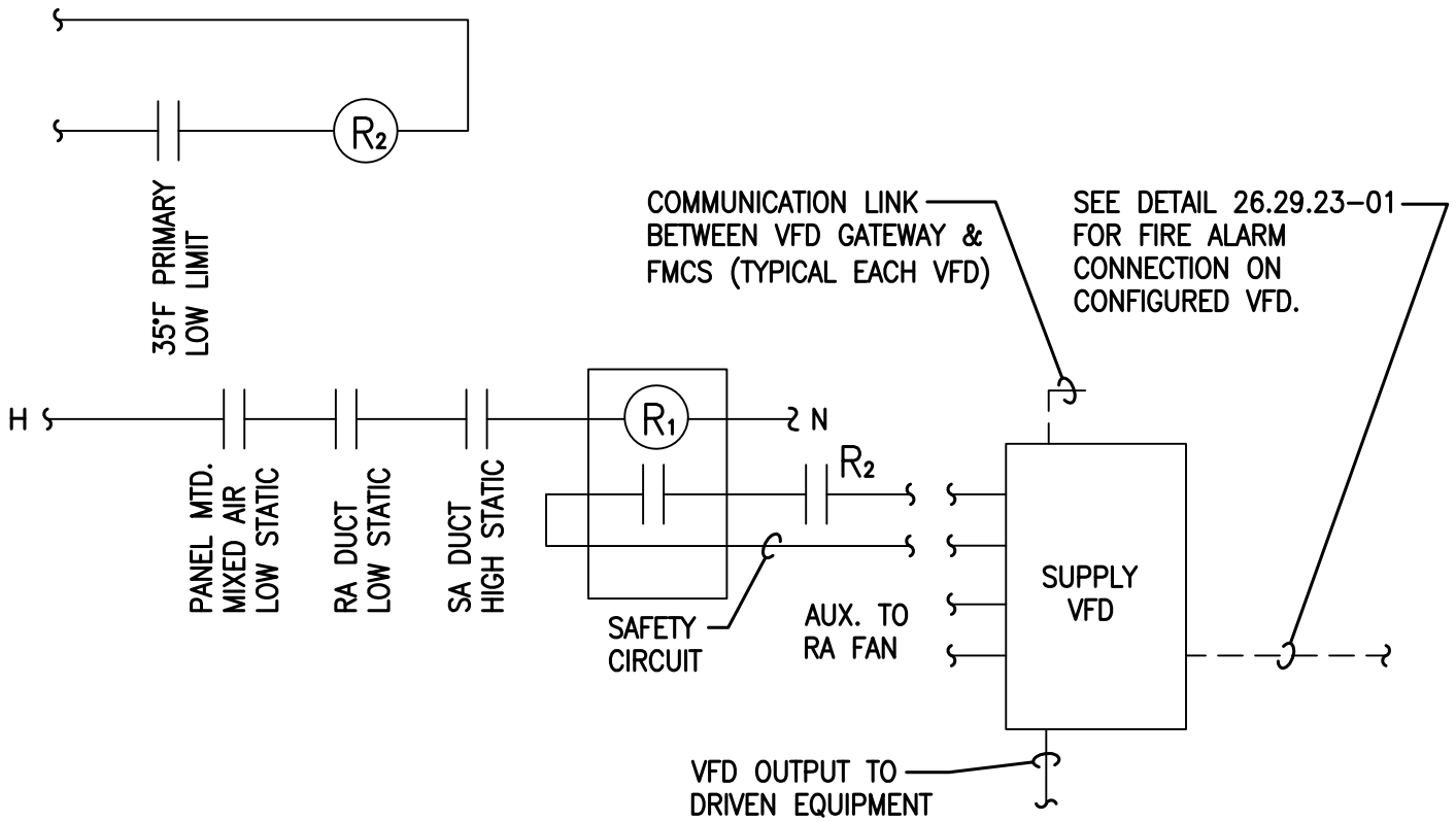
SUPPLY FAN VFD TEMPERATURE CONTROL DIAGRAM
