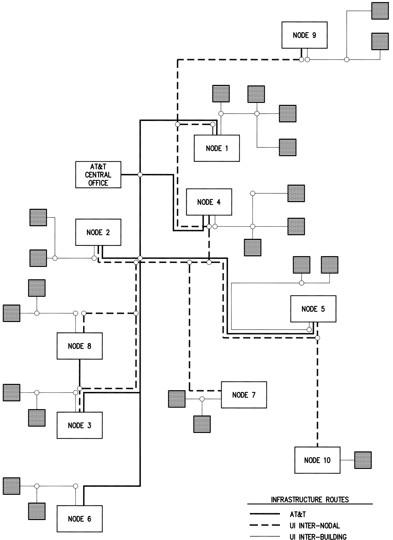
TYPICAL OUTSIDE PLANT DISTRIBUTION DIAGRAM
